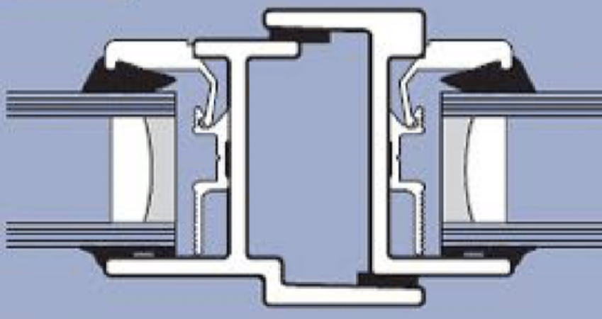
Double leaf meeting stile
