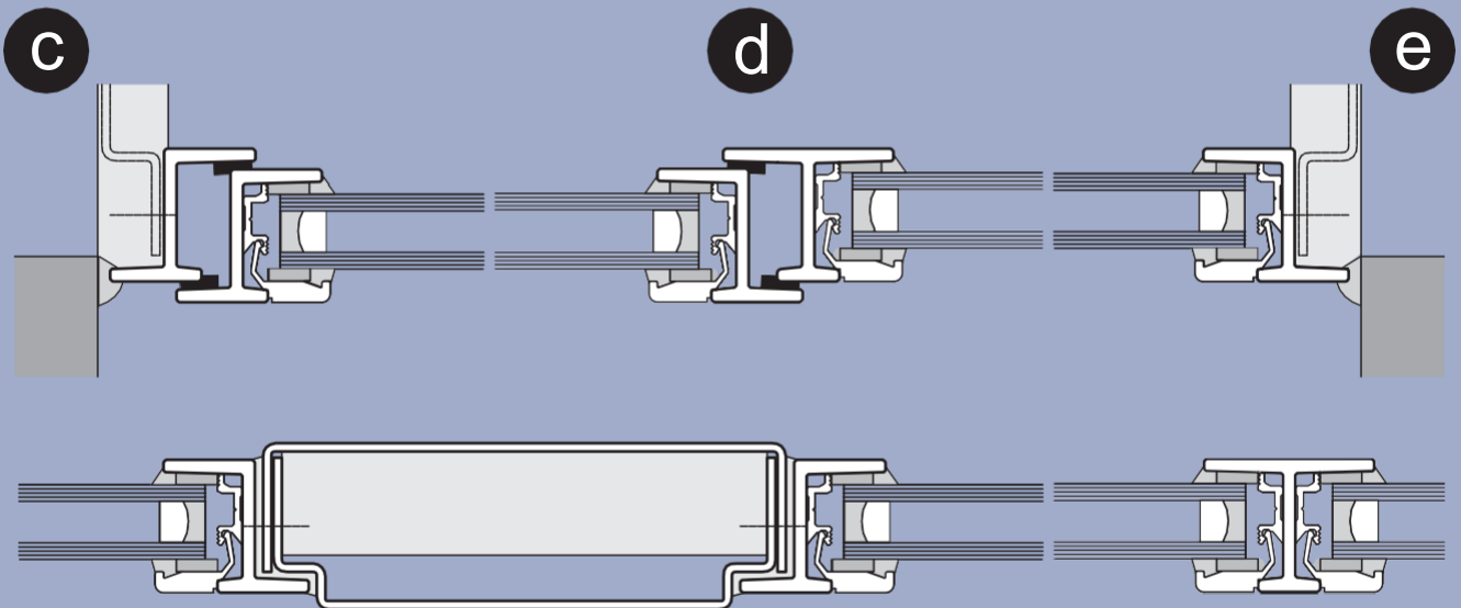
Pressed box mullion (Typical detail - all pressed items are purpose made to suit application)
